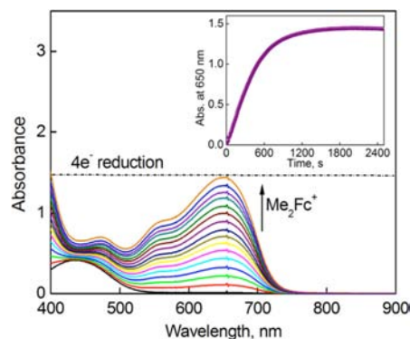
Figure 1. UV–vis spectral changes observed in the four-electron reduction of O_2 (1.0 mM) by Me_2Fc (6.0 mM) with HClO_4 (40 mM) catalyzed by 1 (0.20 mM) in acetone at 298 K. Inset shows the time profile of the absorbance at 650 nm due to Me_2Fc^+ .
