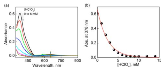
Figure 3. (a) UV–visible spectral changes of [\text{Cu}^{\text{II}}_2(\text{XYLO})(\text{OH})](\text{PF}_6)_2 ( 1 ) (0.20 mM) upon addition of \text{HClO}_4 (0.0–6.0 mM) in acetone at 298 K. (b) Absorbance changes at 378 nm as a function of \text{HClO}_4 concentration.
