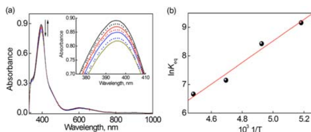
Figure 8. (a) UV-visible spectra indicating the reversible nature of dioxygen binding to [\text{Cu}^{\text{I}}_2(\text{XYLOH})]^{2+} (3). Bubbling \text{O}_2 into an acetone solution of 3 produces [\text{Cu}^{\text{II}}_2(\text{XYLO})(\text{OOH})]^{2+} (4) at 193 K (black, solid line). Increasing the temperature up to 223 K produces dark-yellow solid spectrum. After cooling to 193 K again gives black dotted spectrum. (b) van't Hoff plot to determine the activation parameters, enthalpy and entropy, in the dioxygen binding to [\text{Cu}^{\text{I}}_2(\text{XYLOH})]^{2+} in acetone.
